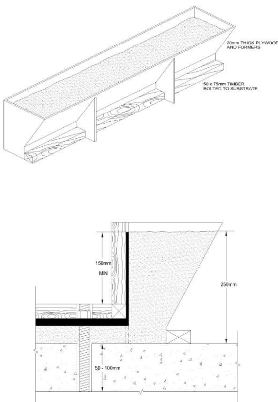
Fig.2 Typical Hopper detail
